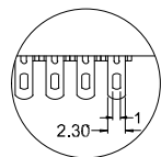
Solder eyelet Type
